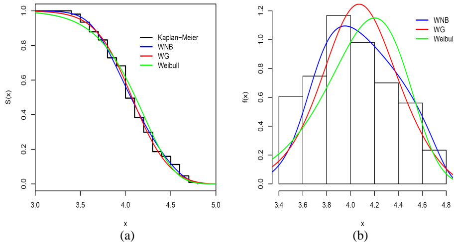
Figure 8. (a) Estimated survival function from the fitted WNB, WG and Weibull distributions and the empirical survival for clorpirifos data. (b) Estimated densities of the WNB, WG and Weibull models for clorpirifos data.
